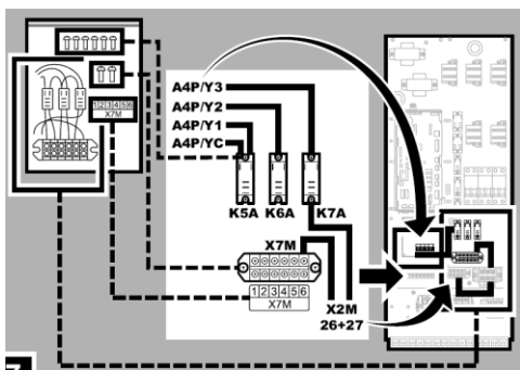
For Hydrobox Installation
